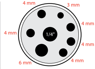
Multi-hole M01
